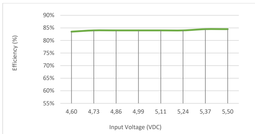
SDM01S0505D, with full Load
