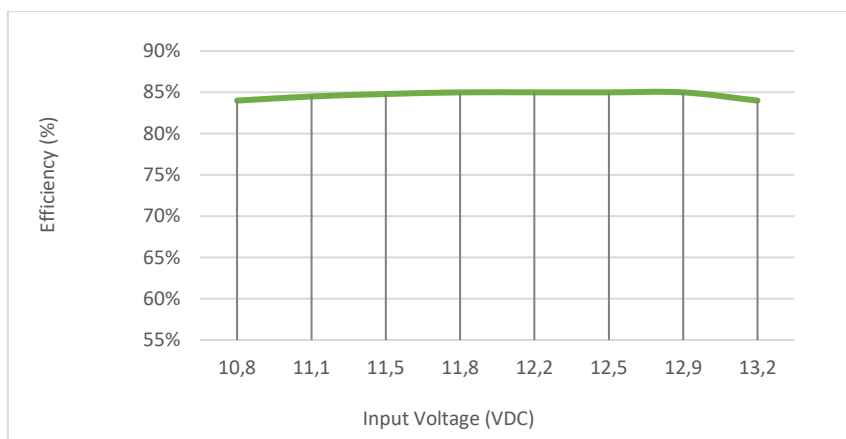
SDM01S1205, with full Load
