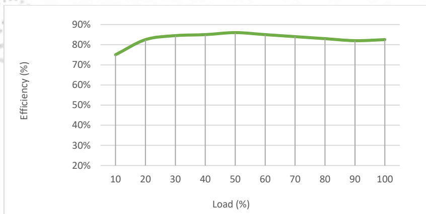
SDM01S0505D, with nominal input voltage
